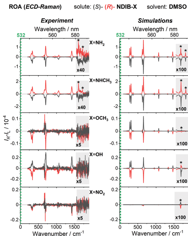
Fig. 4 Experimental (left) and simulated (right) ECD-Raman spectra of NDIB-X derivatives (as shown in Fig. 3) for the DMSO solvent. The intensity of the solute bands is magnified 5, 40 or 100 times and is presented in the grey boxes and marked by asterisks.
