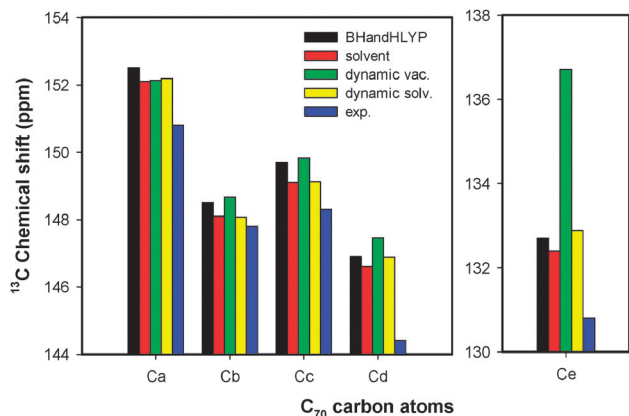
Fig. 4 Importance of various effects on calculated 13 C chemical shifts in C 70 . BHandHLYP stands for shifts obtained by the vacuum BHandHLYP/IGLO-III calculation, “solvent” denotes the BHandHLYP/IGLO-III/CPCM model, and the other bars are related to the involvement of vacuum and solvent FPMD dynamics. All data are corrected for the estimated basis set error calculated from difference between the IGLO-IV and IGLO-III results in Table 1 (all results comprise the previous enhancements, e.g. the “dynamic” = BHandHLYP shifts in vacuum + solvent contribution + basis set correction + dynamic contribution). The experiment is taken from ref. 13.
