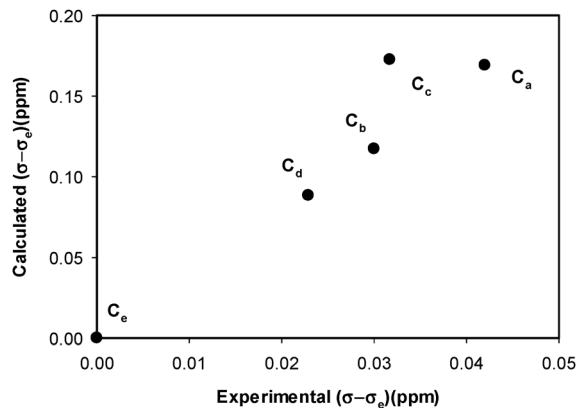
Fig. 5 Temperature effect on NMR shifts in C 70 . Plot shows comparison of experimental and theoretical (BP86/IGLO-II//HF/6-31G) differences in relative shieldings caused by temperature ( \Delta = 100 K). The shift is referenced to C e .
